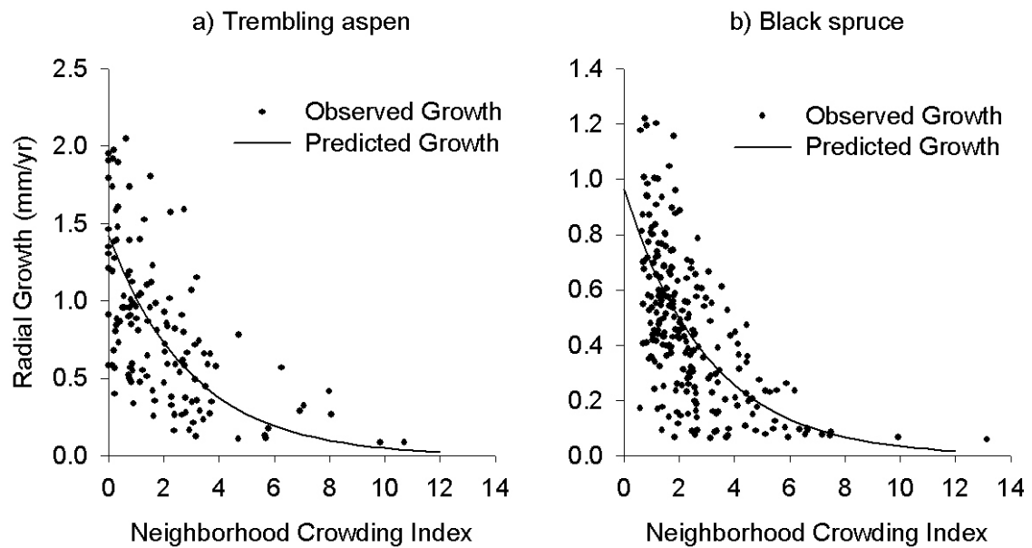
Figure 1.3 : Distribution of observed growth with neighbourhood competition index (NCI) using a) trembling aspen best model and b) black spruce best crowding only model
